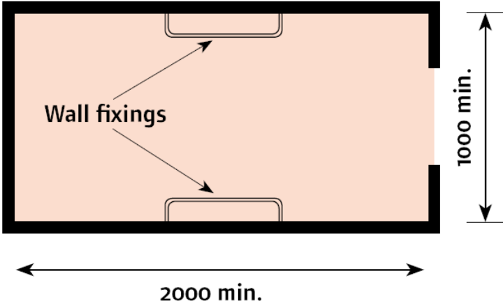
Figure 8: Plan of communal store for four cycles using Sheffield stands 30
