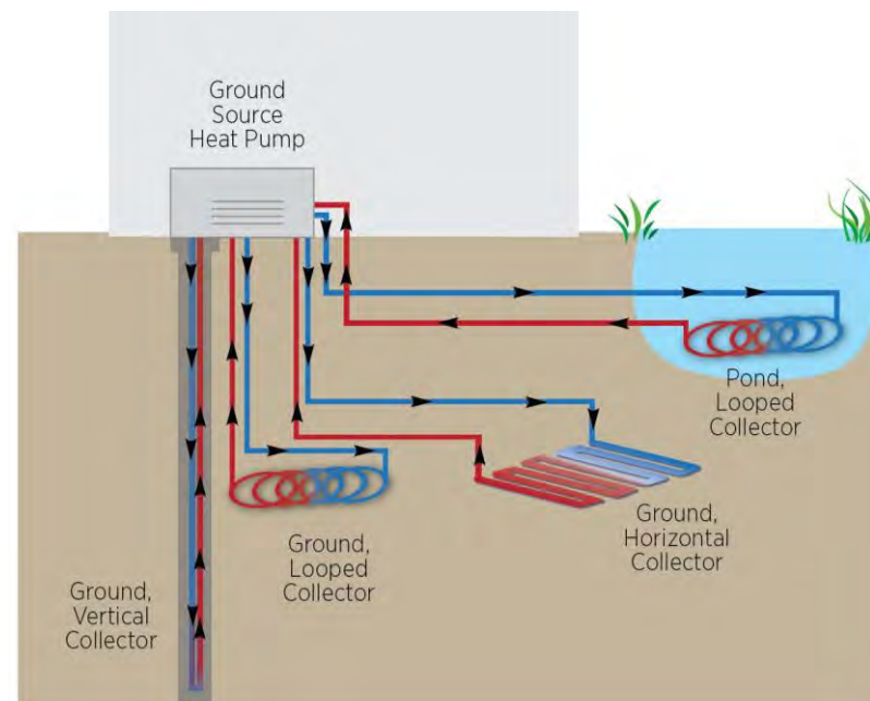
Different types of ground loop can serve the heat pump depending on the space available. (Source: Kete-RVS)
