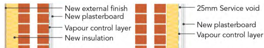
Externally insulated Brick Cavity
